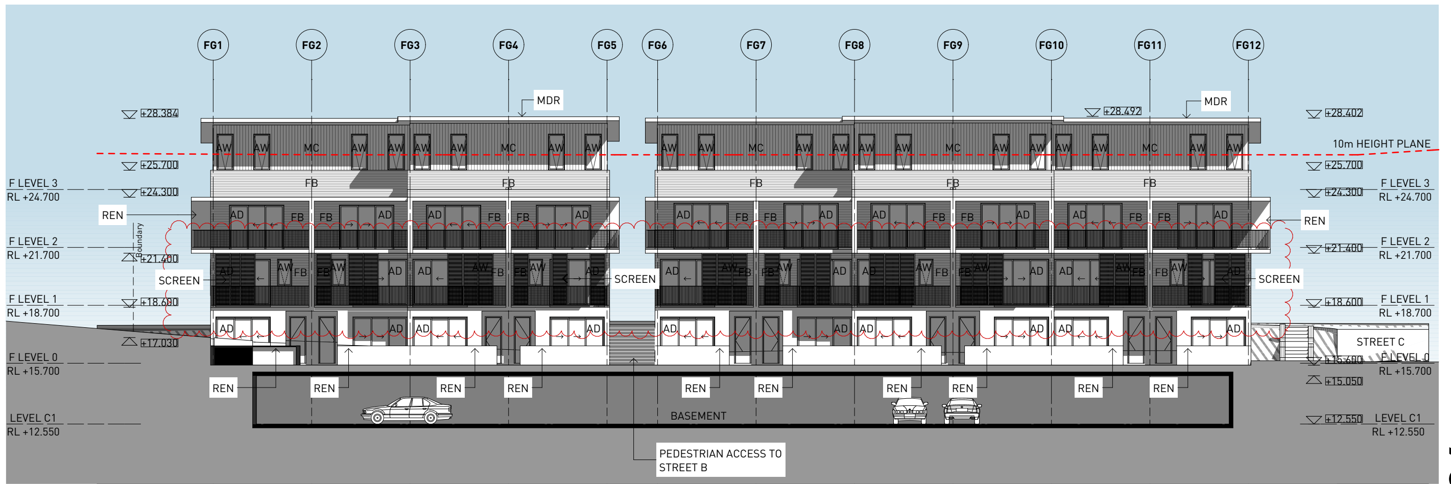
6 WEST ELEVATION BUILDING F 1:200
