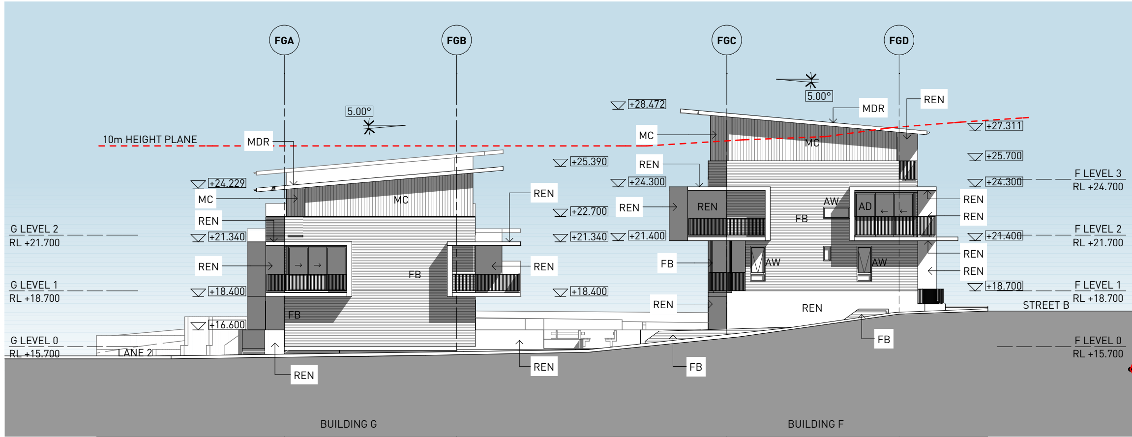
2 SOUTH ELEVATION BUILDING G AND F 1:200
