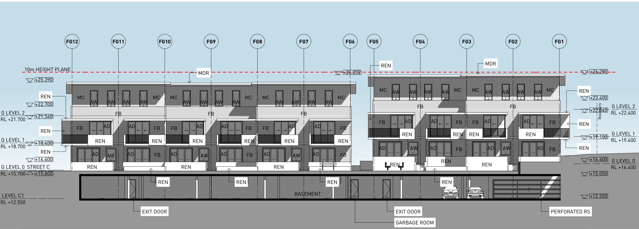
3 EAST ELEVATION BUILDING G 1:200
