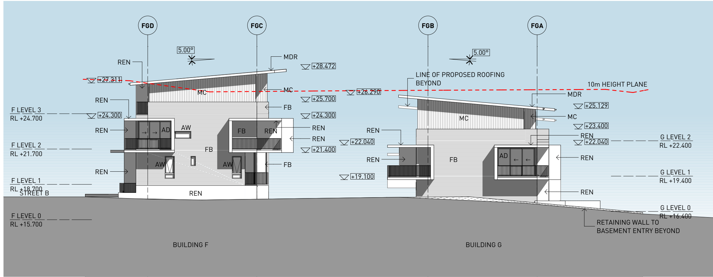
1 NORTH ELEVATION BUILDING G AND F 1:200
